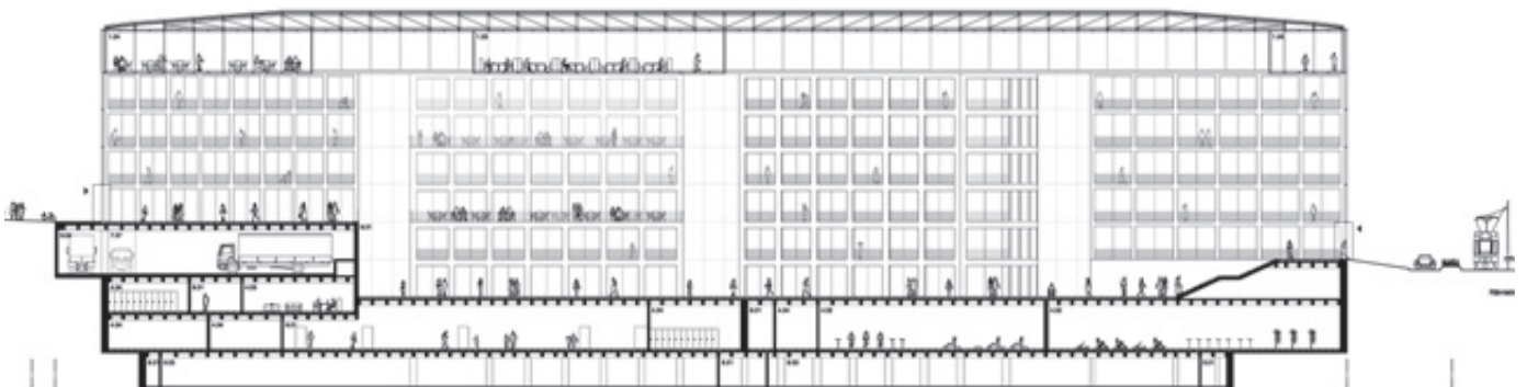
Schnitt Ost-West 1:800
