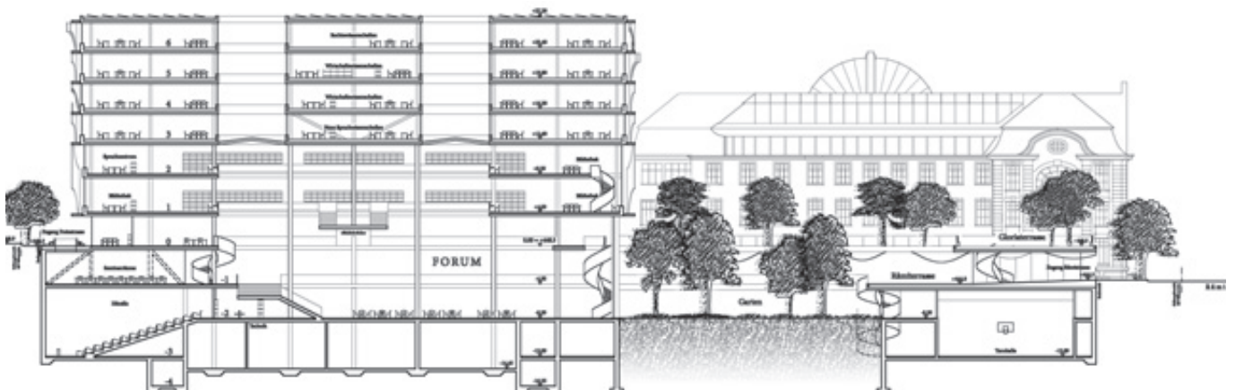
Schnitt Ost-West 1:800
