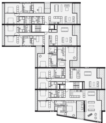
Pianta 6 piano
